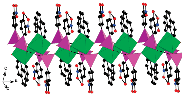
Figure 4. View of the 1D manganese arsonate chain in compound 2. The \text{MnO}_4\text{N}_2 octahedra and \text{AsO}_3 tetrahedra are shaded in green and purple, respectively. N, O, and C atoms are drawn as blue, red, and black circles, respectively. Hydrogen bonds are drawn as dashed lines.
