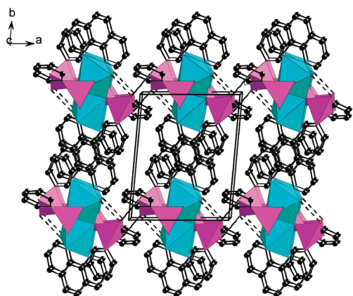
Figure 2. View of the structure of compound 1 down the c axis. The \text{CdO}_4\text{N}_2 octahedra are shaded in cyan, and the \text{AsO}_3 tetrahedra are shaded in purple. O and C atoms are drawn as red and black circles, respectively. Hydrogen bonds are represented by dashed lines.
