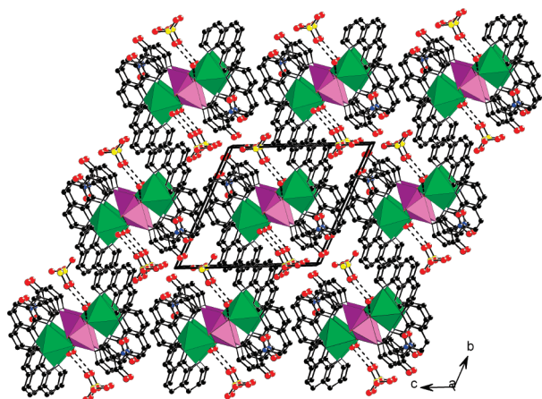
Figure 7. View of the structure of 4 down the a axis. The \text{MnO}_2\text{N}_4 octahedra and \text{CaAsO}_3 tetrahedra are shaded in green and purple, respectively. N, O, C, and Cl atoms are drawn as blue, red, black, and yellow circles, respectively. Hydrogen bonds are drawn as dashed lines.
