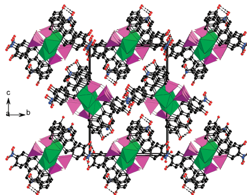
Figure 5. View of the structure of 3 down the a axis. The \text{MnO}_4\text{N}_2 octahedra and \text{AsO}_3 tetrahedra are shaded in green and purple, respectively. N, O, and C atoms are drawn as blue, red, and black circles, respectively. Hydrogen bonds are drawn as dashed lines.
